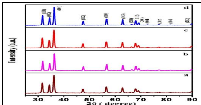
FIG. 1: X-RAY DIFFRACTION OF THE AS-SYNTHESIZED Se DOPED ZnO NANOPARTICLES PREPARED BY CHEMICAL SYNTHESIS METHOD (a) \text{Zn}_{0.95}\text{Se}_{0.05}\text{O}_{1-\delta} ; (b) \text{Zn}_{0.90}\text{Se}_{0.10}\text{O}_{1-\delta} ; (c) \text{Zn}_{0.85}\text{Se}_{0.15}\text{O}_{1-\delta} ; (d) \text{Zn}_{0.80}\text{Se}_{0.20}\text{O}_{1-\delta}
