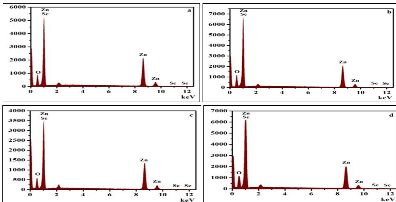
FIG. 5: EDAX SPECTRA OBTAINED ON THE Se DOPED ZnO NANOPARTICLES PREPARED BY CHEMICAL SYNTHESIS METHOD (a) Zn_{0.95}Se_{0.05}O_{1-\delta} ; (b) Zn_{0.90}Se_{0.10}O_{1-\delta} ; (c) Zn_{0.85}Se_{0.15}O_{1-\delta} ; (d) Zn_{0.80}Se_{0.20}O_{1-\delta}
