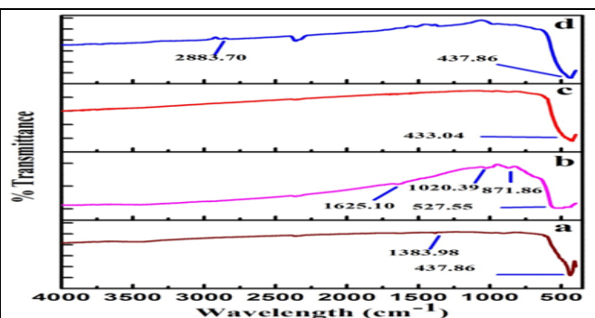
FIG. 2: FTIR SPECTRA OBTAINED ON THE Se DOPED ZnO NANOPARTICLES PREPARED BY CHEMICAL SYNTHESIS METHOD (a) \text{Zn}_{0.95}\text{Se}_{0.05}\text{O}_{1-\delta} ; (b) \text{Zn}_{0.90}\text{Se}_{0.10}\text{O}_{1-\delta} ; (c) \text{Zn}_{0.85}\text{Se}_{0.15}\text{O}_{1-\delta} ; (d) \text{Zn}_{0.80}\text{Se}_{0.20}\text{O}_{1-\delta}
