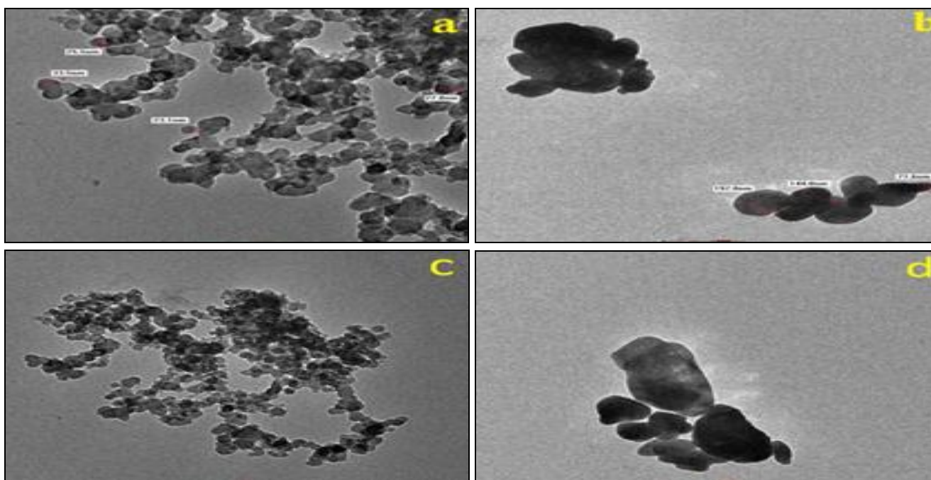
FIG. 6: (a, b, c AND d) TEM IMAGES OBTAINED ON Zn_{0.80}Se_{0.20}O_{1-\delta} NANOPARTICLES PREPARED BY CHEMICAL SYNTHESIS METHOD
