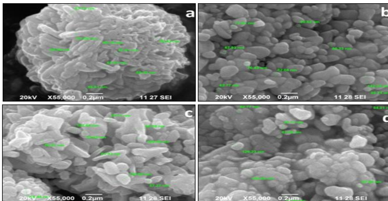
FIG. 4: SEM PHOTOGRAPHS OBTAINED ON THE Se DOPED ZnO NANOPARTICLES PREPARED BY CHEMICAL SYNTHESIS METHOD (a) Zn_{0.95}Se_{0.05}O_{1-\delta} ; (b) Zn_{0.90}Se_{0.10}O_{1-\delta} ; (c) Zn_{0.85}Se_{0.15}O_{1-\delta} ; (d) Zn_{0.80}Se_{0.20}O_{1-\delta}
