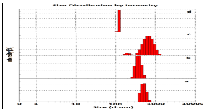
FIG. 3: PARTICLE SIZE CHARACTERISTIC CURVES OBTAINED ON THE Se DOPED ZnO NANOPARTICLES PREPARED BY CHEMICAL SYNTHESIS METHOD (a) \text{Zn}_{0.95}\text{Se}_{0.05}\text{O}_{1-\delta} ; (b) \text{Zn}_{0.90}\text{Se}_{0.10}\text{O}_{1-\delta} ; (c) \text{Zn}_{0.85}\text{Se}_{0.15}\text{O}_{1-\delta} ; (d) \text{Zn}_{0.80}\text{Se}_{0.20}\text{O}_{1-\delta}
