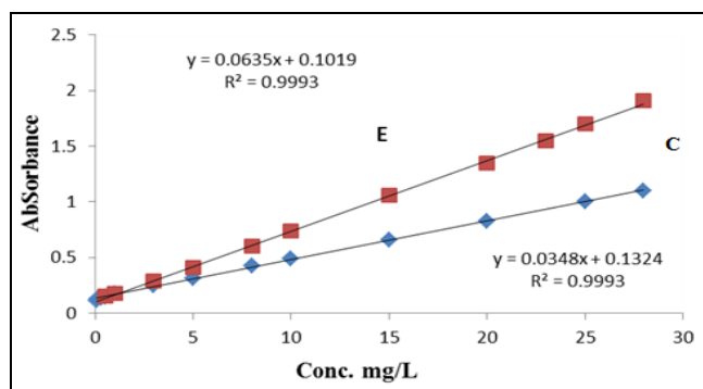
FIG. 9: CALIBRATION CURVE OF VITAMIN C AND E
