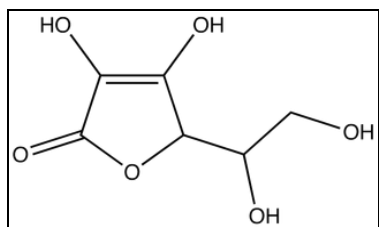
FIG. 1: CHEMICAL STRUCTURE OF VITAMIN C
