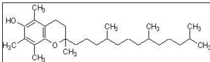
FIG. 2: CHEMICAL STRUCTURE OF VITAMIN E ( \alpha -TOCOPHEROL)
