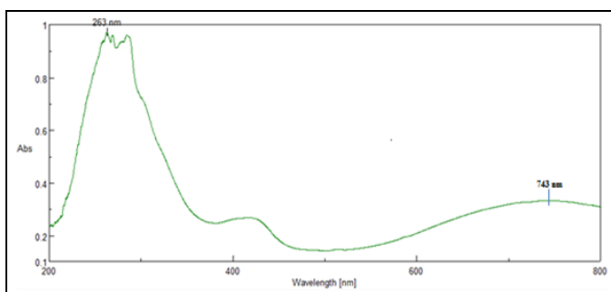
FIG. 3: ABSORPTION SPECTRA OF VITAMIN (C OR E), K_3Fe(CN)_6 AND FeNH_4(SO_4)_2 MIXTURE
