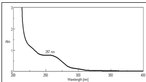
FIG. 1: UV ABSORPTION SPECTRUM OF OLMESARTAN IN METHANOL
