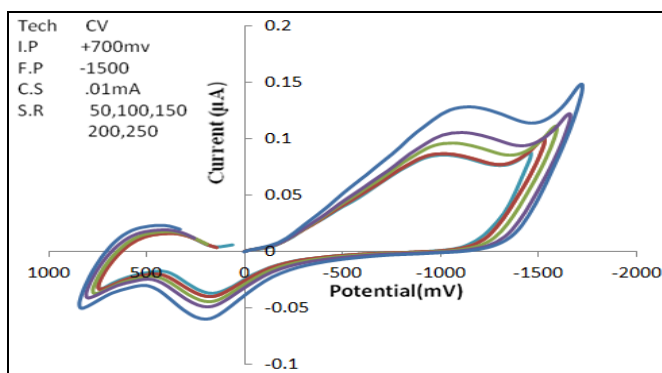
FIG. 3: CYCLIC VOLTAMMOGRAMS OF GBAPI IN METHANOLIC MEDIUM CONTAINING PHOSPHATE BUFFER (pH 8)
