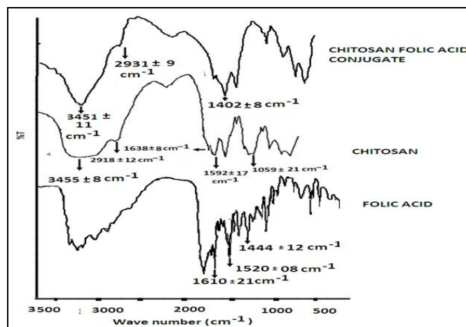
FIG. 2: PEAKS OF CHITOSAN FOLIC ACID CONJUGATE, CHITOSAN, AND FOLIC ACID
