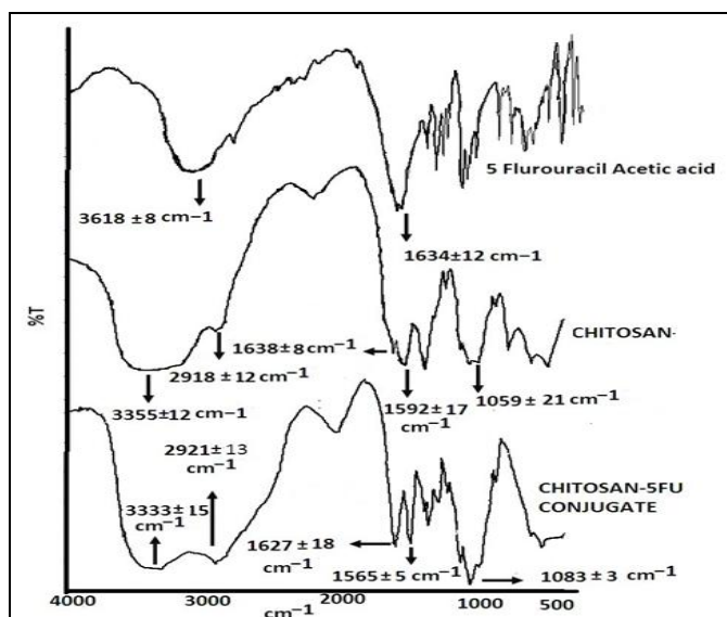
FIG. 4: 5 FLUROURACIL-1-YL-ACETIC ACID AND CHITOSAN-5 FLUROURACIL CONJUGATE AND CHARACTERISTIC PEAKS ASSIGNMENT OF CHITOSAN
