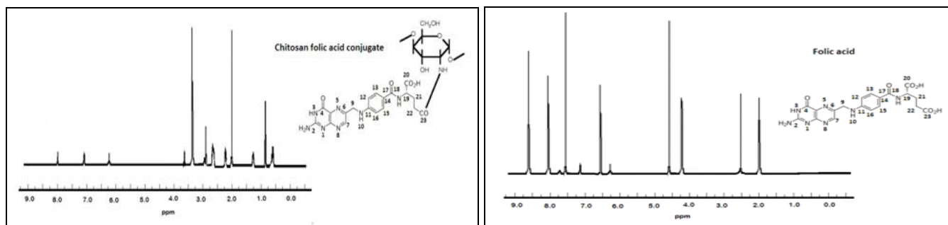
FIG. 3: NMR SPECTRUM OF CHITOSAN FOLIC ACID CONJUGATE AND FOLIC ACID
