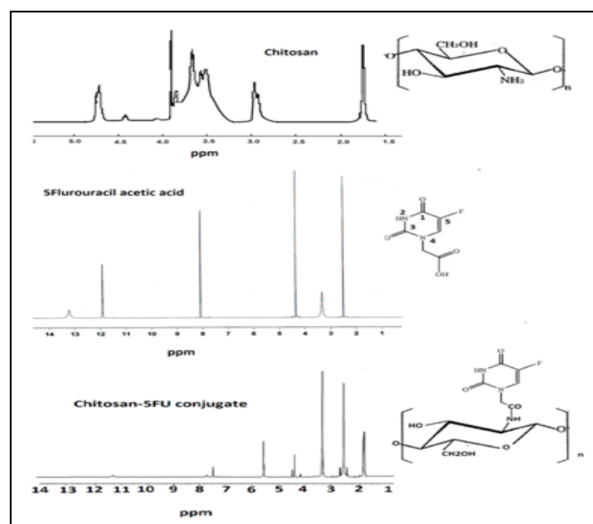
FIG. 5: CHITOSAN, 5 FLUROURACIL-1-YL ACETIC ACID AND CHITOSAN-5 FLUROURACIL CONJUGATE
