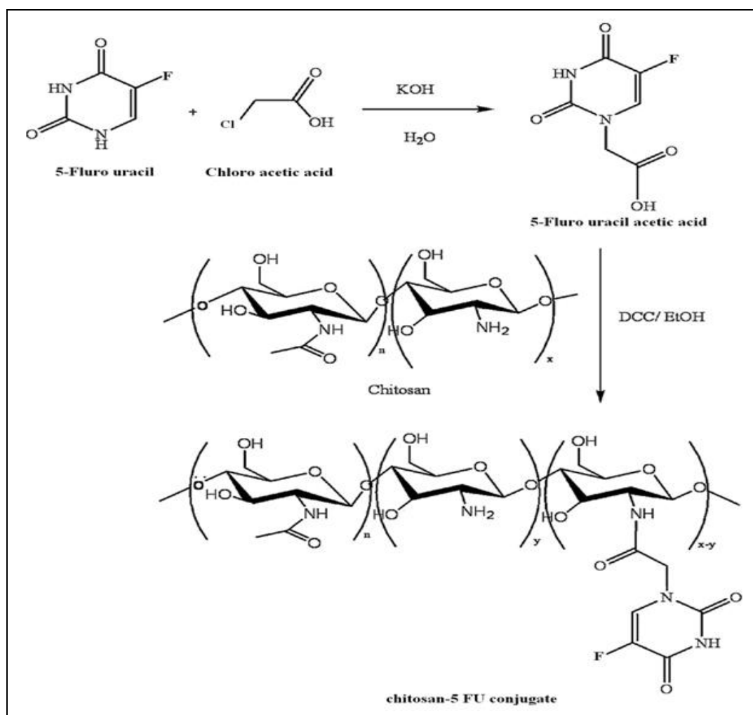
FIG. 1: PREPARATION OF CHITOSAN-5 FU ACETIC ACID CONJUGATE
