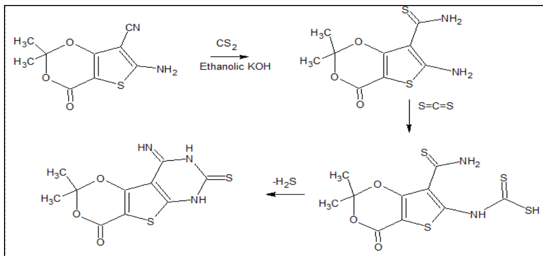
9-imino-2,2-dimethyl-7-thioxo-6,9-dihydro-4H,7H-[1,3]dioxino[4',5':4,5]thieno[2,3-d][1,3]thiazin-4-one
