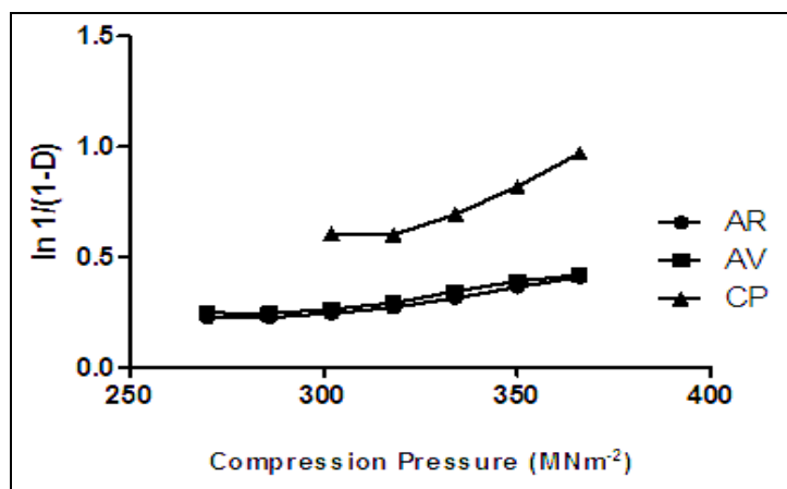
FIG. 1: HECKEL PLOTS FOR EVG COMPACTS PRODUCED USING SELECTED DILUENTS AND GLT (5%W/V) AS BINDER
