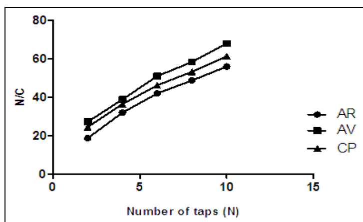
FIG. 2: KAWAKITA PLOTS FOR EVG COMPACTS PRODUCED USING SELECTED DILUENTS AND GLT (5%W/V) USED AS BINDER
