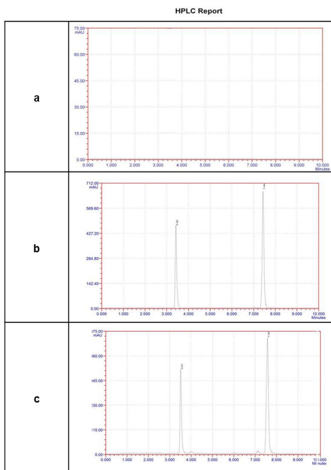
FIGURE 3: CHROMATOGRAM OF (a) BLANK, (b) STANDARD AND (c) FIXED DOSE FORMULATION OF BUPROPION AND NALTREXONE HCl
