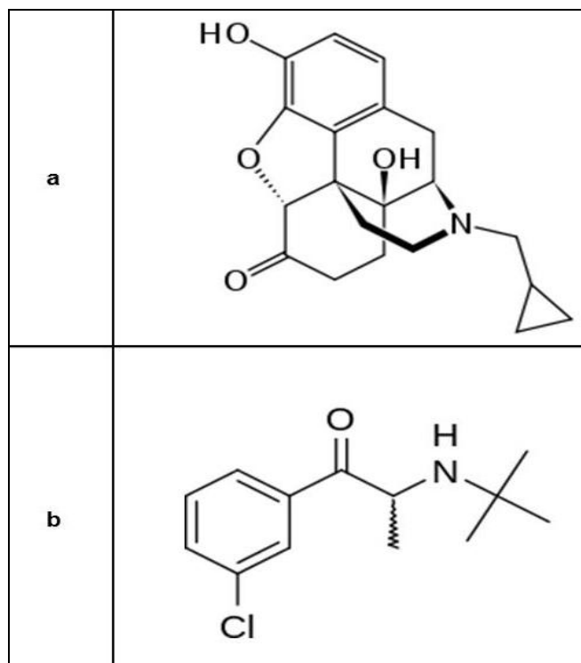
FIG.1: CHEMICAL STRUCTURE OF (a) NALTREXONE AND (b) BUPROPION
