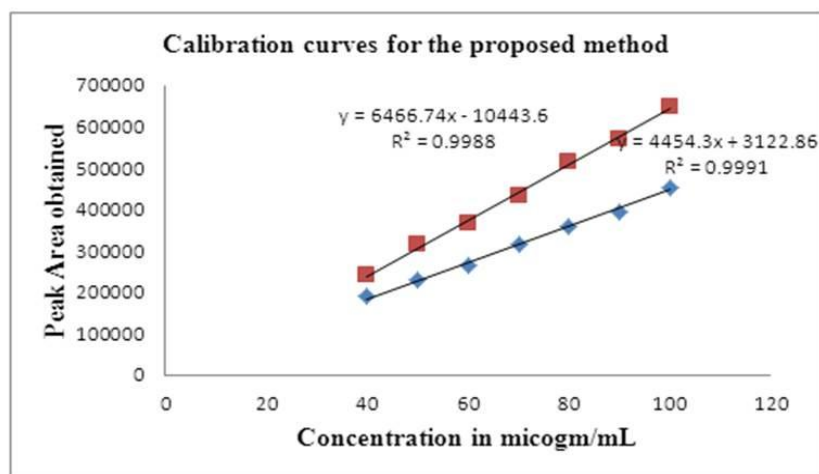
FIGURE 2: LINEARITY GRAPH FOR BUPROPION HCl AND NALTREXONE HCl
