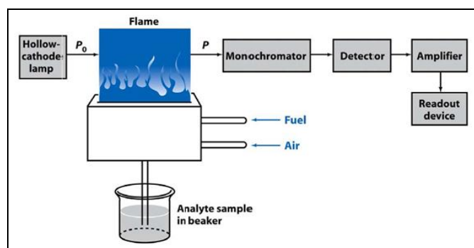
FIG. 4: INSTRUMENT PROCESSES OF AN ATOMIC ABSORPTION SPECTROMETER
