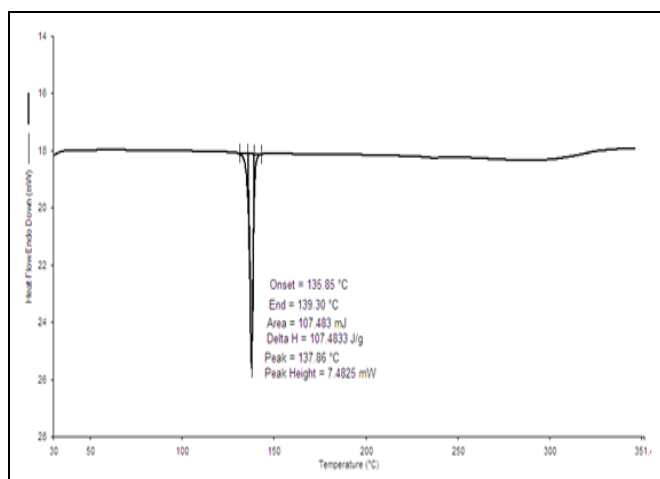
FIG. 5: DSC OF ZOLMITRIPTAN
