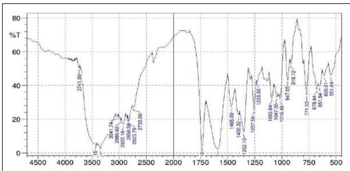
FIG. 3: FTIR OF ZOLMITRIPTAN
