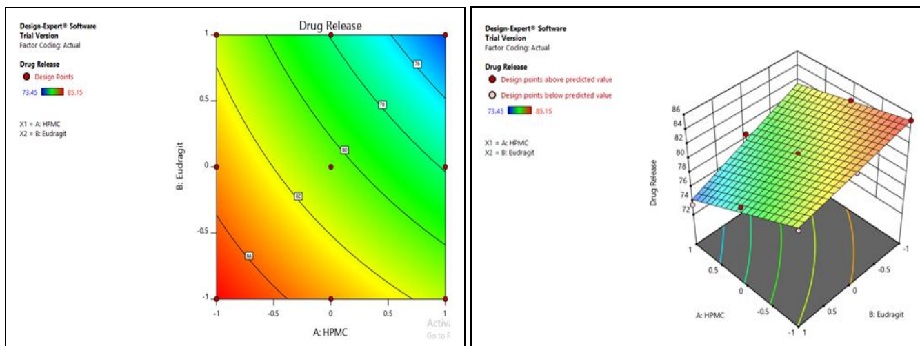
FIG. 10: THE RESPONSE SURFACE GRAPH FOR % DRUG RELEASE PRODUCT Y2
