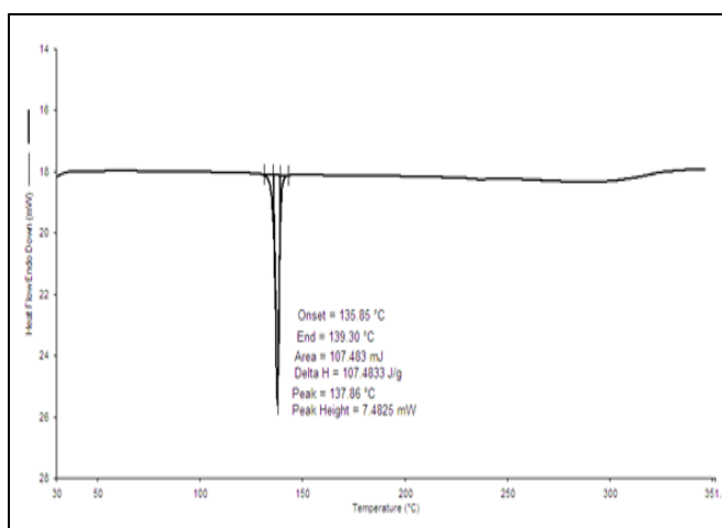
FIG. 6: DSC OF DRUG AND EXCIPIENTS
