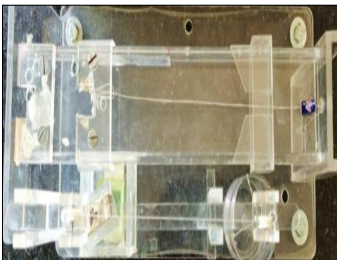
FIG. 1B: TOP VIEW OF MUCOADHESION TESTER
