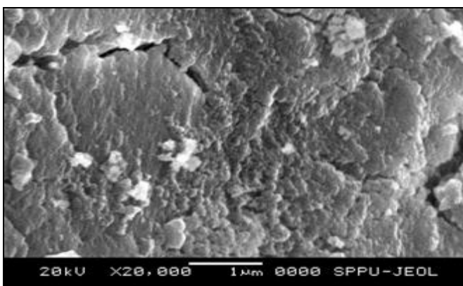
FIG. 5: SEM IMAGE OF AS PREPARED NICKEL OXIDE NANOCLUSTERS CAPPED WITH TBPB (0.01M) AT 5 MA/ \text{cm}^2 CURRENT DENSITY
