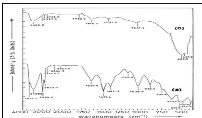
FIG. 2: FTIR SPECTRA OF NICKEL OXIDE SYNTHESIZED AT 5 MA \text{cm}^{-2} CURRENT DENSITY AND USING TBPB AS CAPPING AGENT (A) AS PREPARED (B) ANNEALED AT 500 °C
