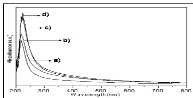
FIG. 1: UV-VISIBLE SPECTRA OF AS PREPARED SAMPLE OF NIO NANOCLUSTERS SYNTHESIZED USING TBPB AS CAPPING AGENT (0.01M) DISPERSED IN WATER AT A: 5, B: 10, C: 15, D: 20 MA/CM 2
