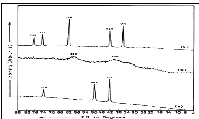
FIG. 3: XRD PATTERNS OF (A) PURE NICKEL METAL (B) NICKEL OXIDE SYNTHESIZED USING TBPB AS CAPPING AGENT AT 5 MA \text{cm}^{-2} CURRENT DENSITY (C) AFTER ANNEALING AT 500 °C
