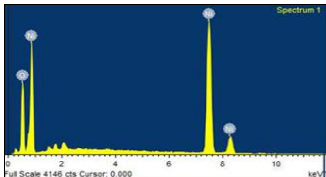
FIG. 6: EDS SPECTRUM OF AS PREPARED NICKEL OXIDE NANOCLUSTERS
