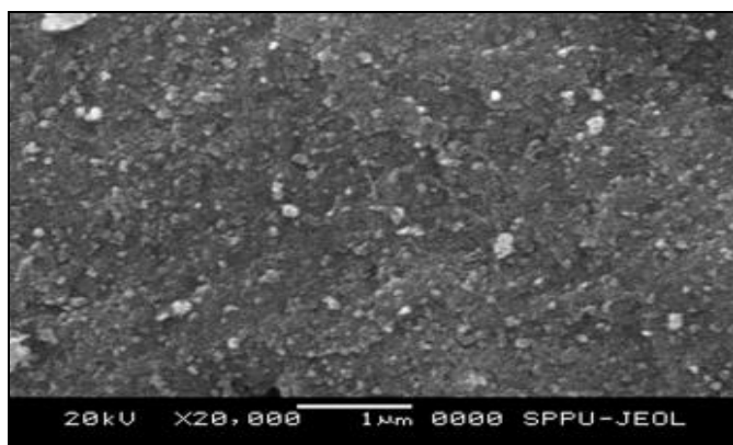
FIG. 4: SEM IMAGE OF AS PREPARED NICKEL OXIDE NANOCLUSTERS CAPPED WITH TBPB (0.01M) AT 10 MA/ \text{cm}^2 CURRENT DENSITY
