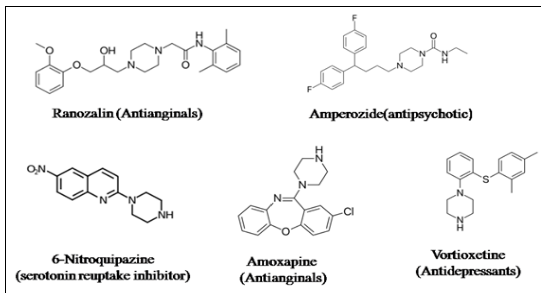
FIG. 1: PIPERAZINE CONJUGATED DRUG MOLECULES
