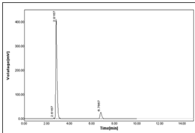
FIG. 7: PEROXIDE DEGRADATION
