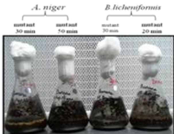
FIG. 12: SOLID STATE FERMENTED BANANA PEEL USING MUTANTS
