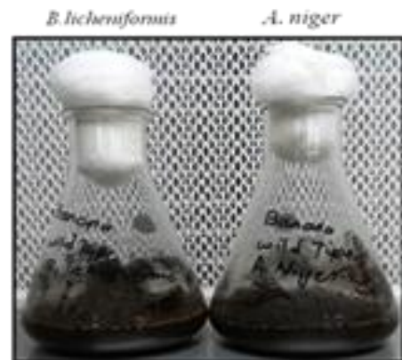
FIG. 10: SOLID STATE FERMENTED BANANA PEEL WASTES USING WILD TYPE MICROORGANISMS
