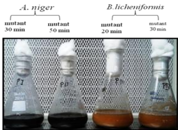
FIG. 17: SUPERNATANT (CRUDE ENZYME) COLLECTED AFTER CENTRIFUGATION OF FERMENTED POTATO PEEL WASTES BY MUTANTS
