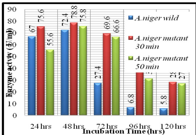
GRAPH 3: EFFECT OF INCUBATION TIME ON ENZYME ACTIVITY USING POTATO AS SUBSTRATE BY A. NIGER
