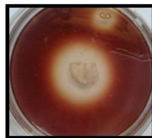
FIG. 5: ZONE OF INHIBITION SHOWN BY BACILLUS LICHENIFORMIS
