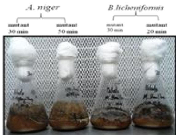
FIG. 13: SOLID STATE FERMENTED POTATO PEEL USING MUTANTS
