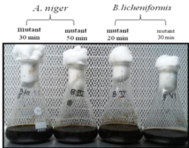
FIG. 16: SUPERNATANT (CRUDE ENZYME) COLLECTED AFTER CENTRIFUGATION OF FERMENTED BANANA PEEL WASTES BY MUTANTS
