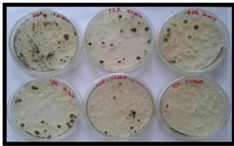
FIG. 6: GROWTH OF MUTATED ASPERGILLUS NIGER
