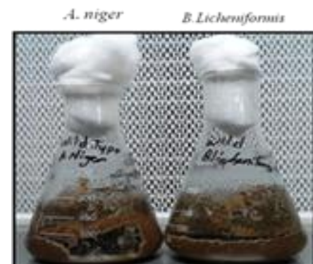
FIG. 11: SOLID STATE FERMENTED POTATO PEEL WASTES USING WILD TYPE MICROORGANISMS
