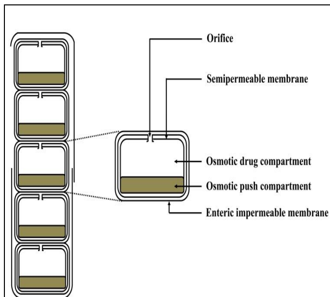
FIG.3: CROSS-SECTION OF THE OROS-CT COLON TARGETED DRUG DELIVERY SYSTEM
