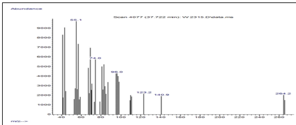
MS OF ARISTOLACTAM 2 IN AQUEOUS EXTRACT (m/z=264.2)
